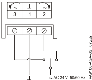
Figure 10: VA9104-AGA-3S Control Wiring Diagram
