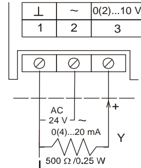
Figure 12: VA9104-GGA-3S Control Wiring Diagram
