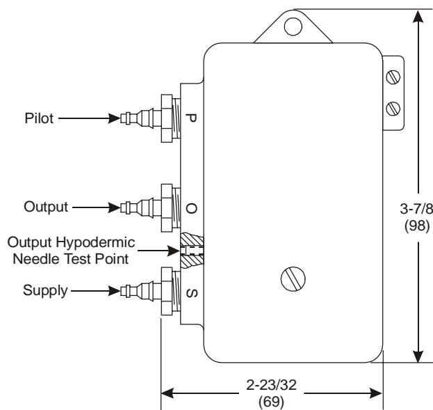
Figure 1: V-9502 Port Identification and Dimensions, in. (mm)
