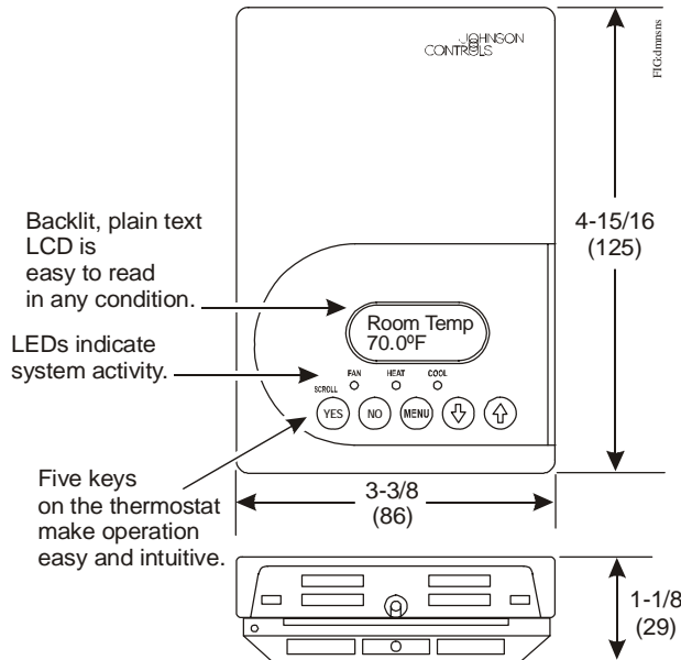
T600xxx-3 Series Thermostats Front Cover
