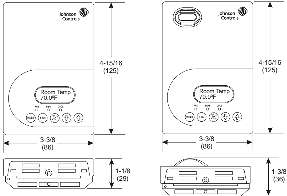
T60xDFH-3 Series Thermostat Controller (Left) and T60xDFH-3+PIR Series Thermostat Controller (Right) Dimensions, in. (mm)
