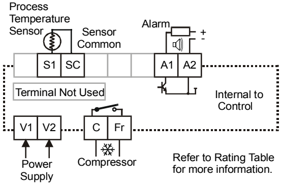
Figure 1: MR1 DIN Rail Mount Control
