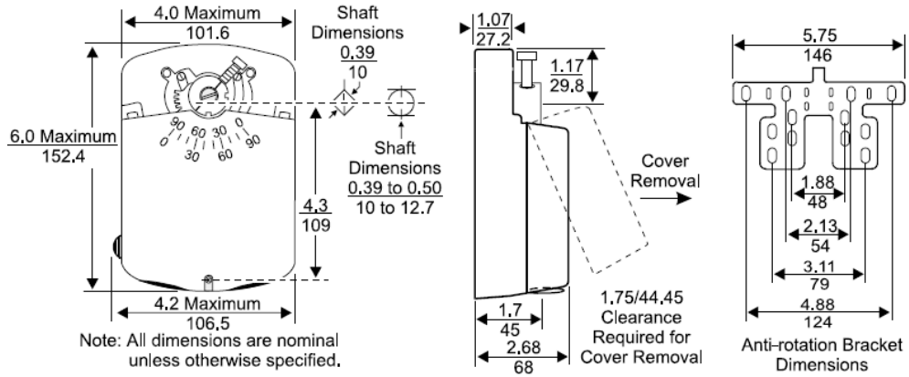
Dimensions, in./mm
