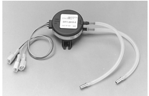
Figure 1: DPT-2015 Differential Pressure Transmitter
