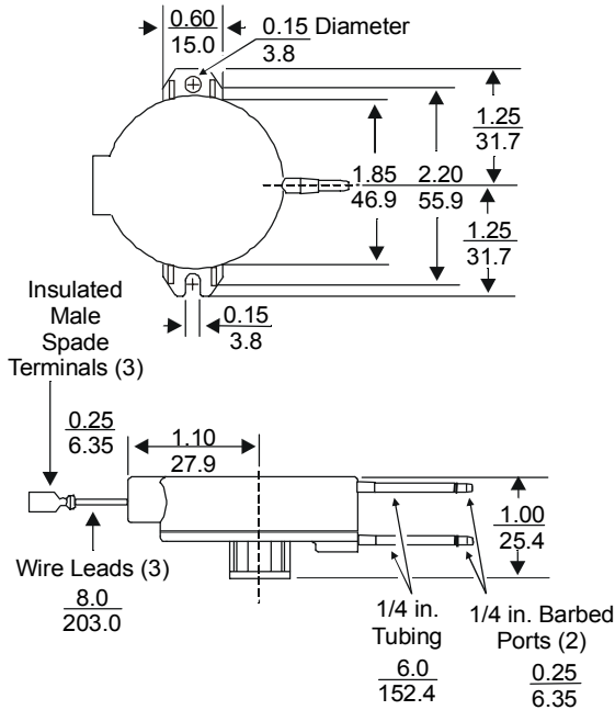
Figure 5: DPT-2015 Dimensions, in. (mm)
