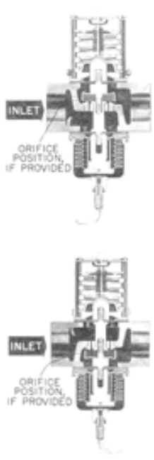
Fig. 2 -- Typical cross-sections of threaded type valves. Interiors of flange models are similar.
