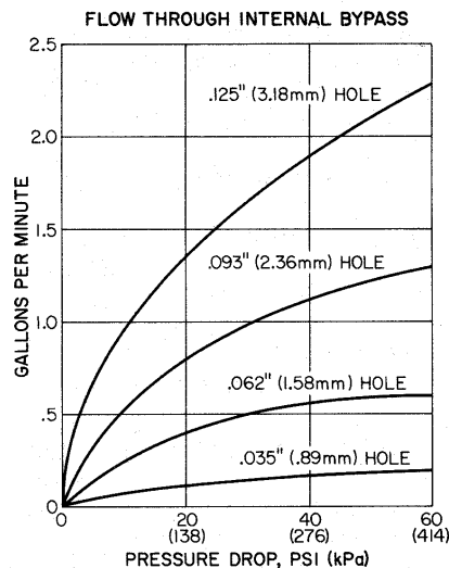
Fig. 4 — Internal Bypass chart.
