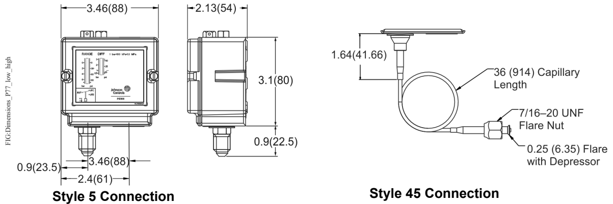
Figure 1: Dimensions of P77 High Pressure Control with Type 1 Enclosure, in. (mm)
